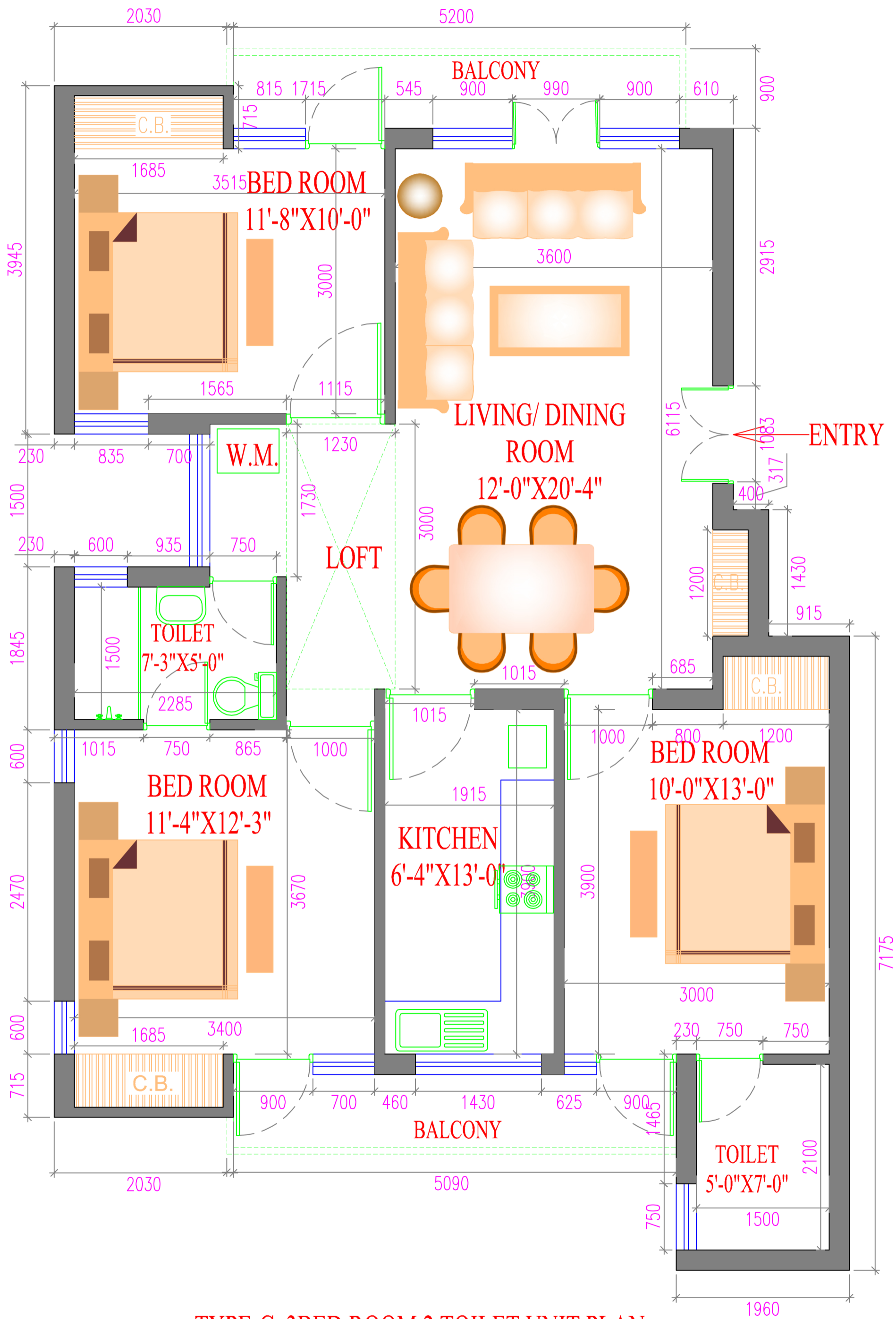
TYPE-C, 3BED ROOM 2 TOILET UNIT PLAN
